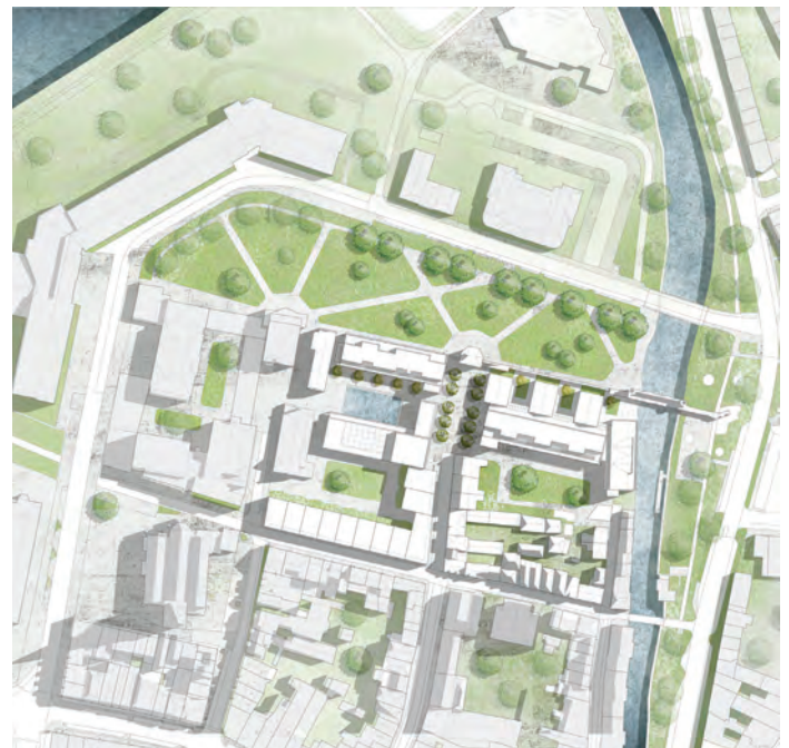
master plan - after intervention
