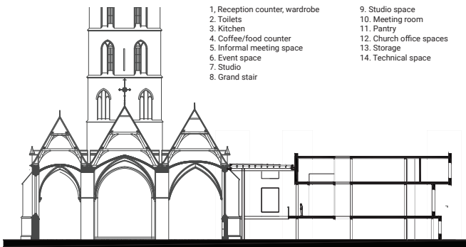
PLANS AND SECTION B
