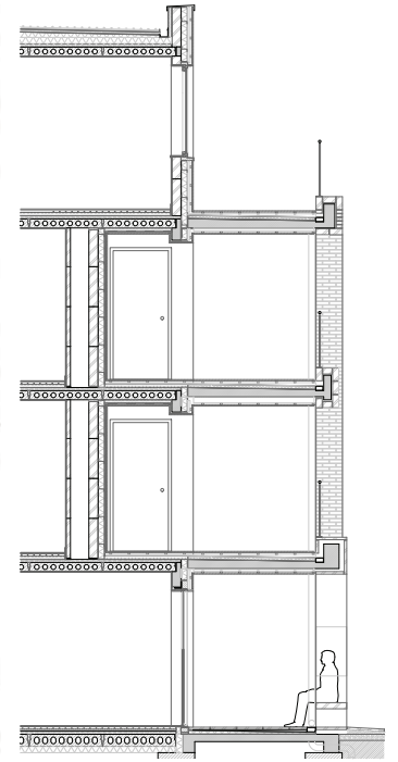
west facade renovation 1:20
